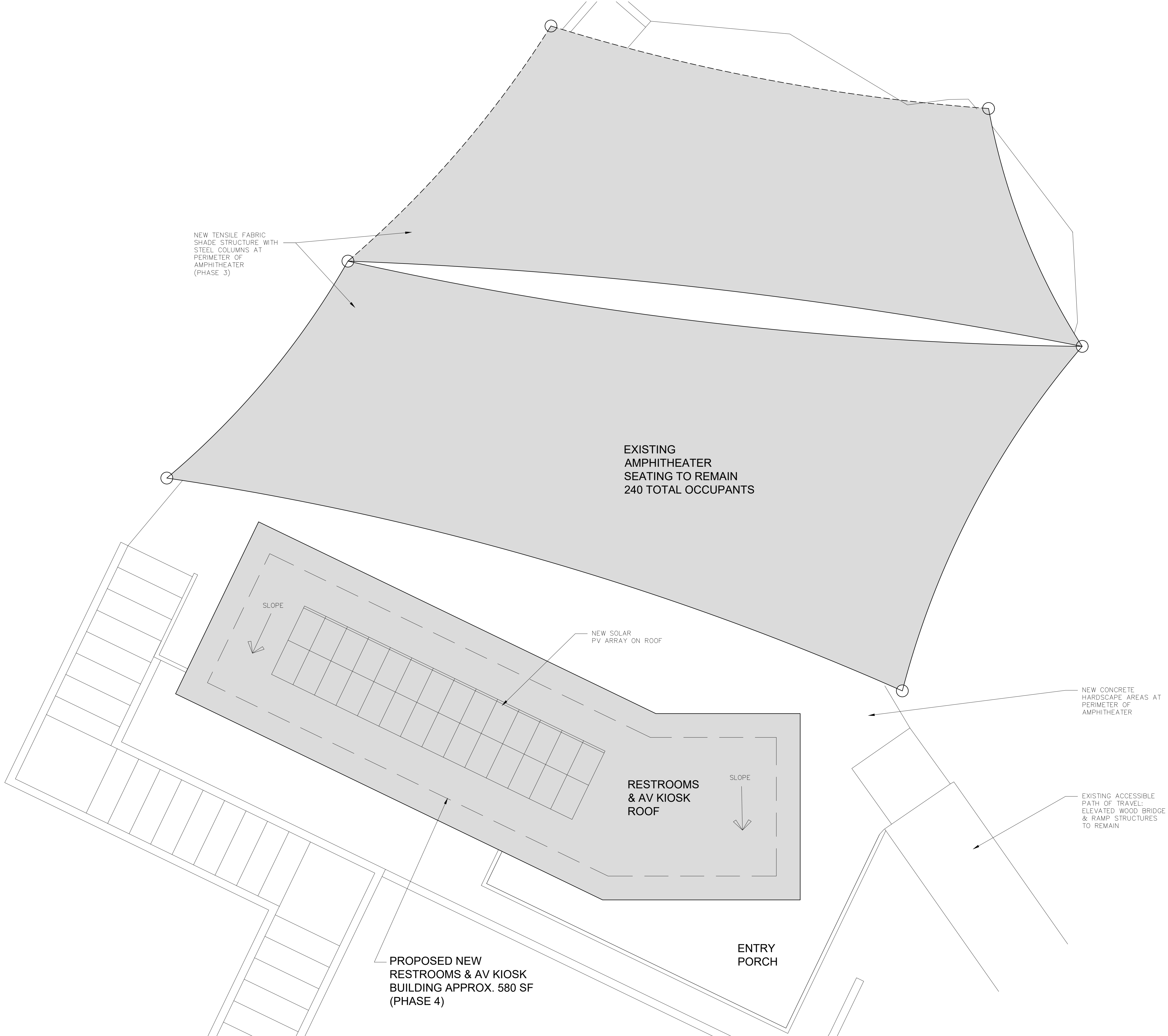
NEW ROOF PLAN - UUFSD AMPHITHEATER
